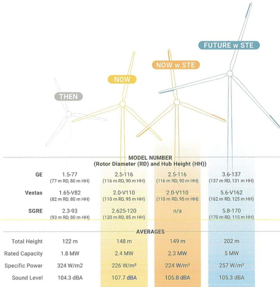
Fig. 5. Then, Now, Now with STE, and Future with STE wind turbine models for each manufacturer. Sound level refers to SWL.
