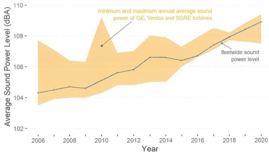
Fig. 2. Annual US fleetwide average and minimum and maximum sound power levels for General Electric (GE), Vestas, and Siemens Gamesa Renewable Energy (SGRE) wind turbines installed in that year, based on data provided to the authors by these manufacturers and data collected as part of the development of the US Wind Turbine Database [26,27]. GE, Vestas, and SGRE constitute 95% of US installed capacity over this period.
