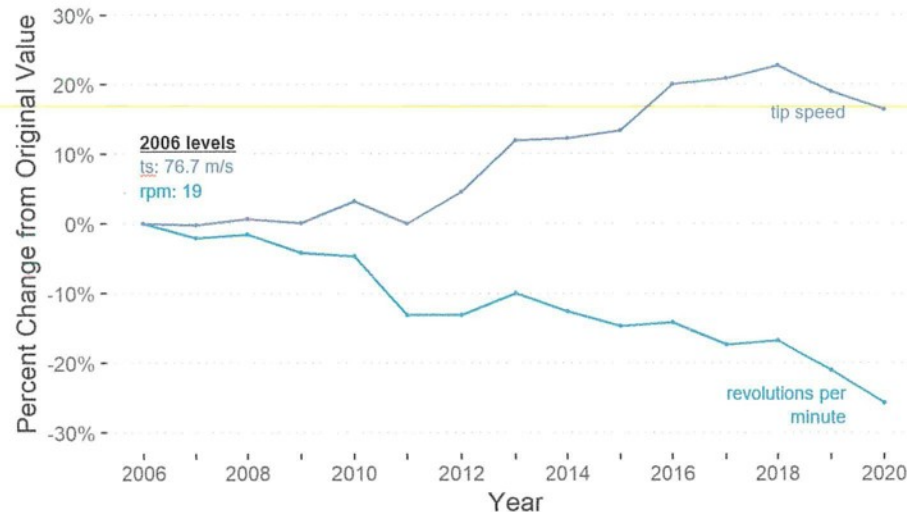
Fig. 3. Average annual fleetwide US wind turbine tip speed (ts) and revolutions per minute (rpm) percentage change trends over time. 2006 original levels shown at left. Source: Based on calculations derived from data collected for Wiser et al., 2022 from manufacturers turbine brochures.
